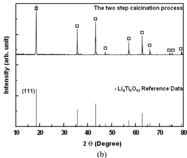
Fig. 2. XRD curve of as-synthesized (a) pseudo-LTO and (b) LTO powders.
