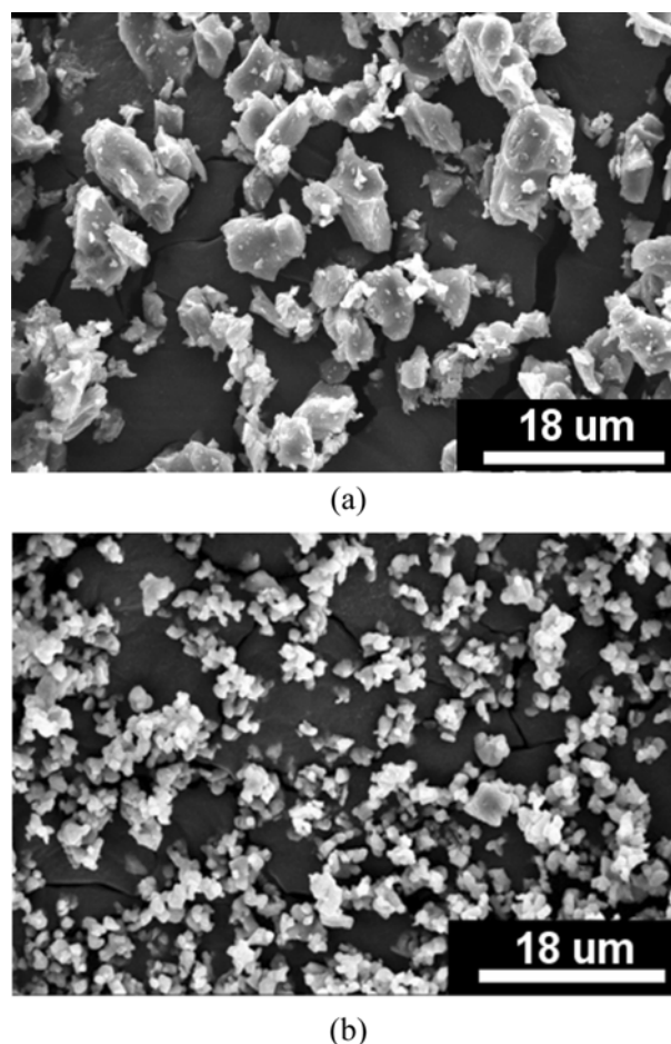
Fig. 4. FESEM images of the pseudo-LTO (a) and the LTO (b) powders.
